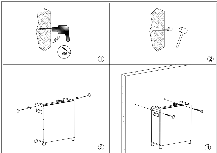
Fig.6-1 Fix the Brackets to the Battery
