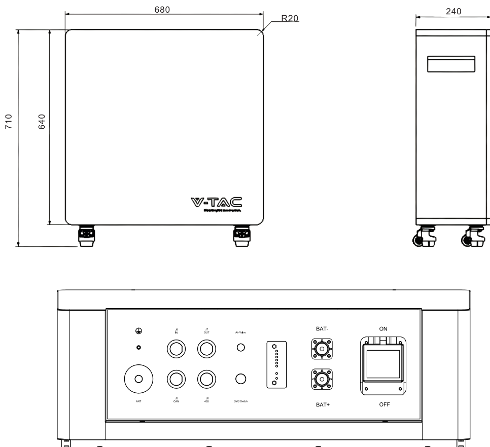
Fig. 5-1 Product Dimensions
